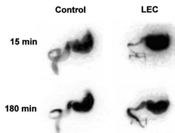
Figure 1. Reconstructed pictures of whole body PET. The three-dimensional PET scans were reconstructed to two-dimensional images. Shown are the time frames from 0 to 15 min and from 165–180 min after copper administration for a control rat and an LEC rat. The bar corresponds to 1 cm and the resolution is 0.5 mm. Movies of these PET scans can be found at www.ikp.unibe.ch/pet .
